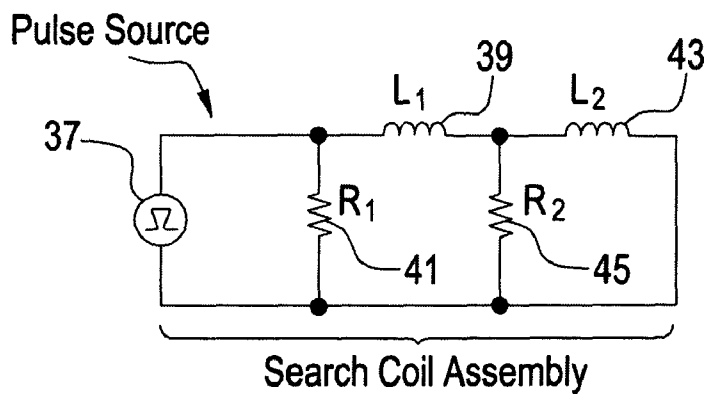
Wiring Diagram 2 Coil Assembly
