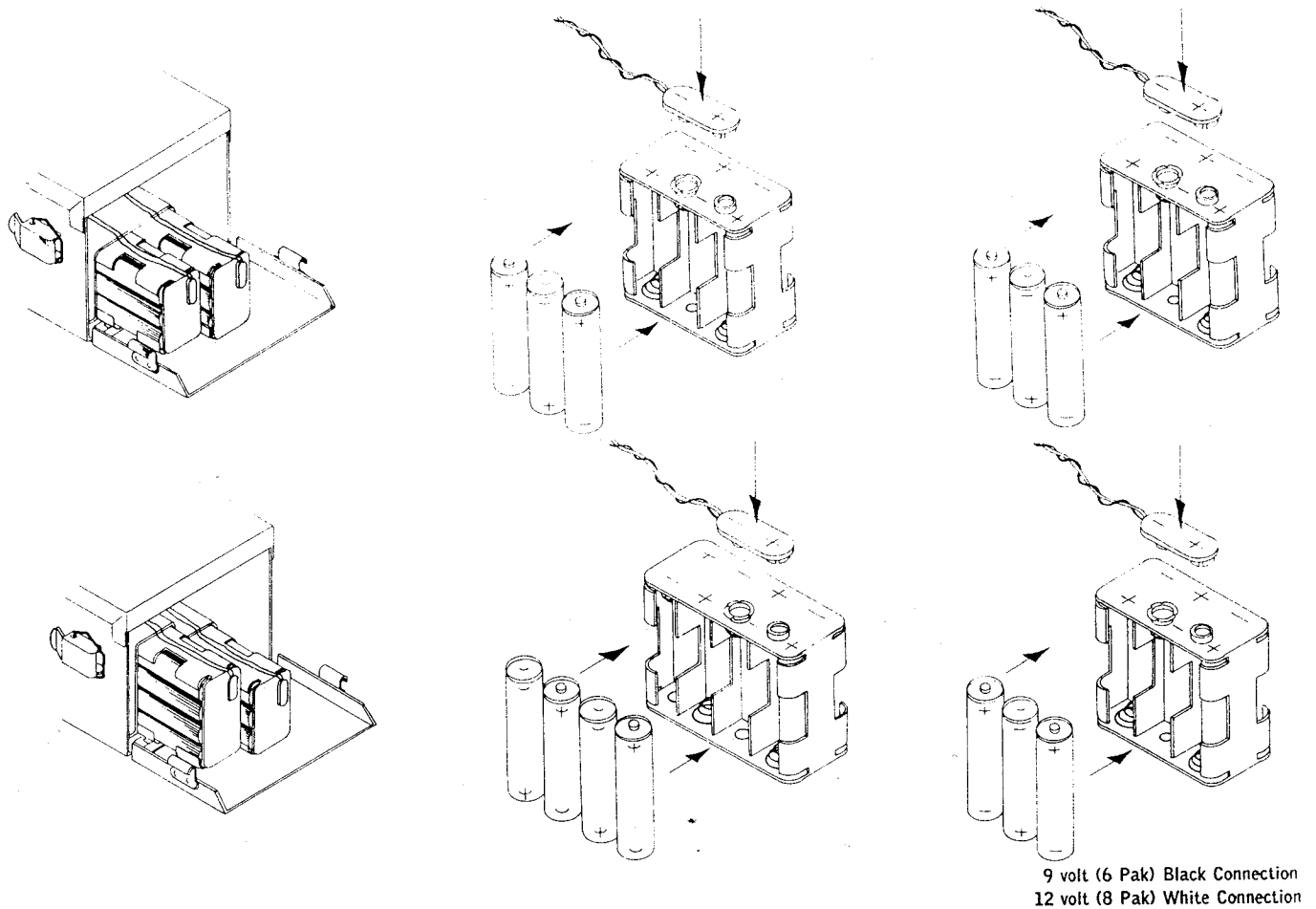
BATTERY-PACK ILLUSTRATION
