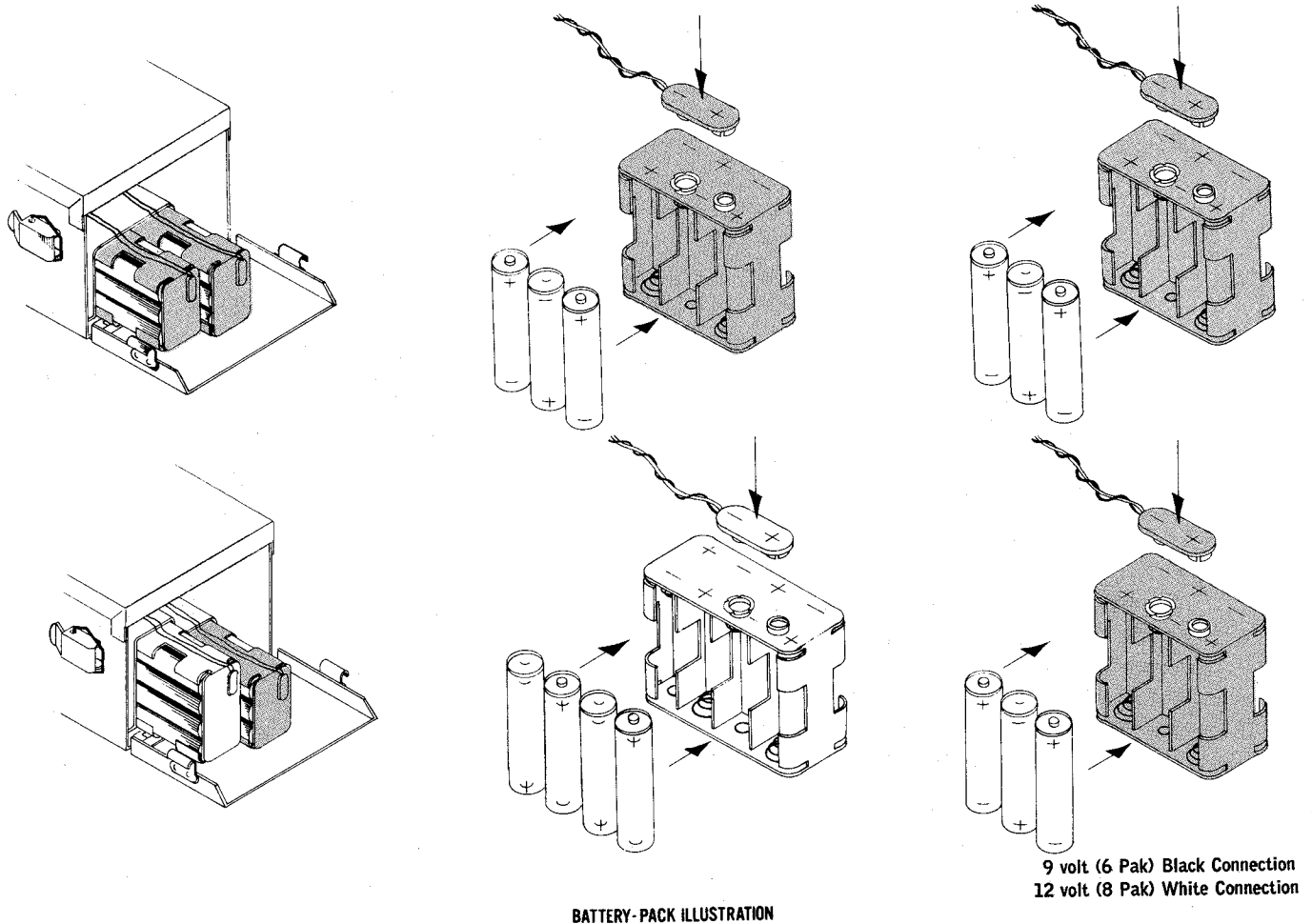
BATTERY-PACK ILLUSTRATION
