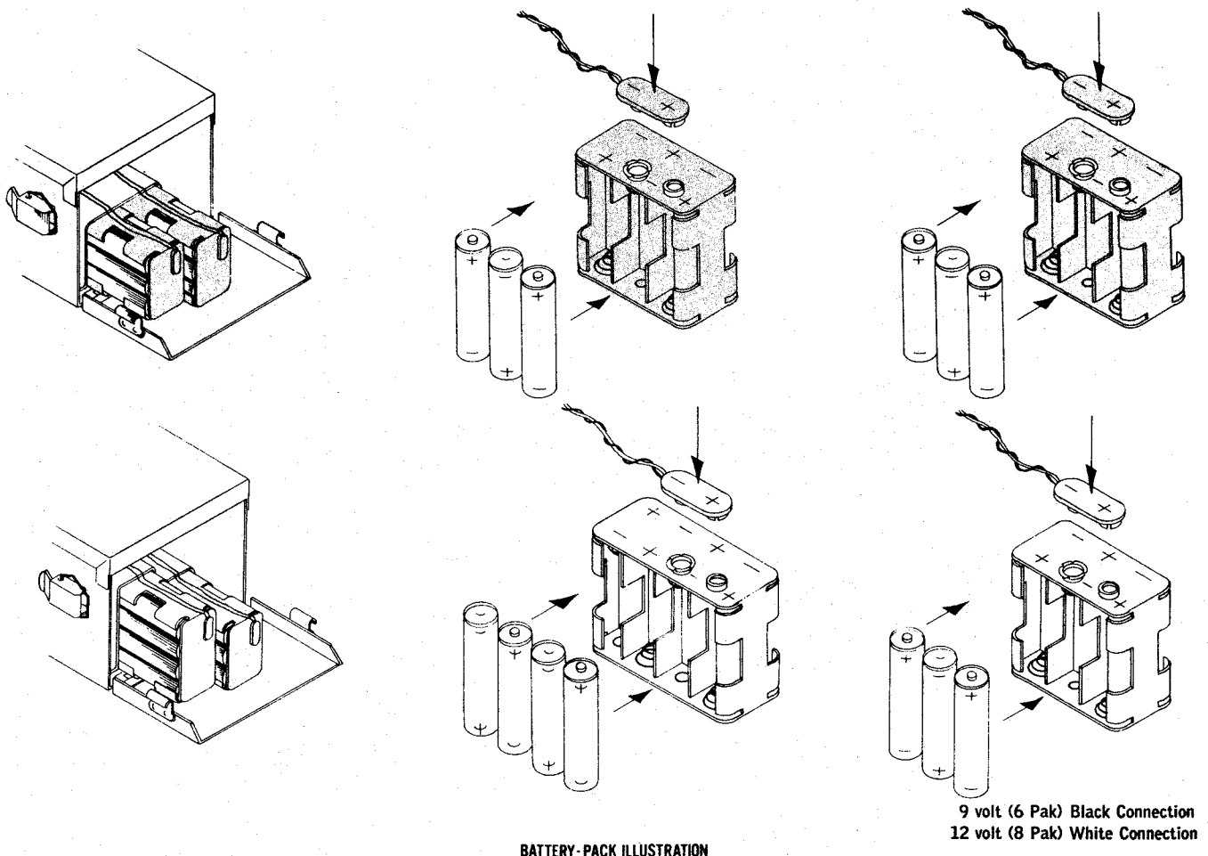
BATTERY-PACK ILLUSTRATION
