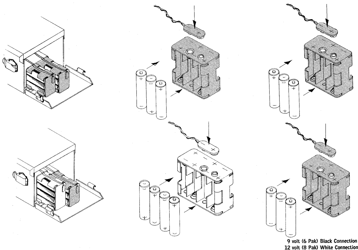
BATTERY-PACK ILLUSTRATION
