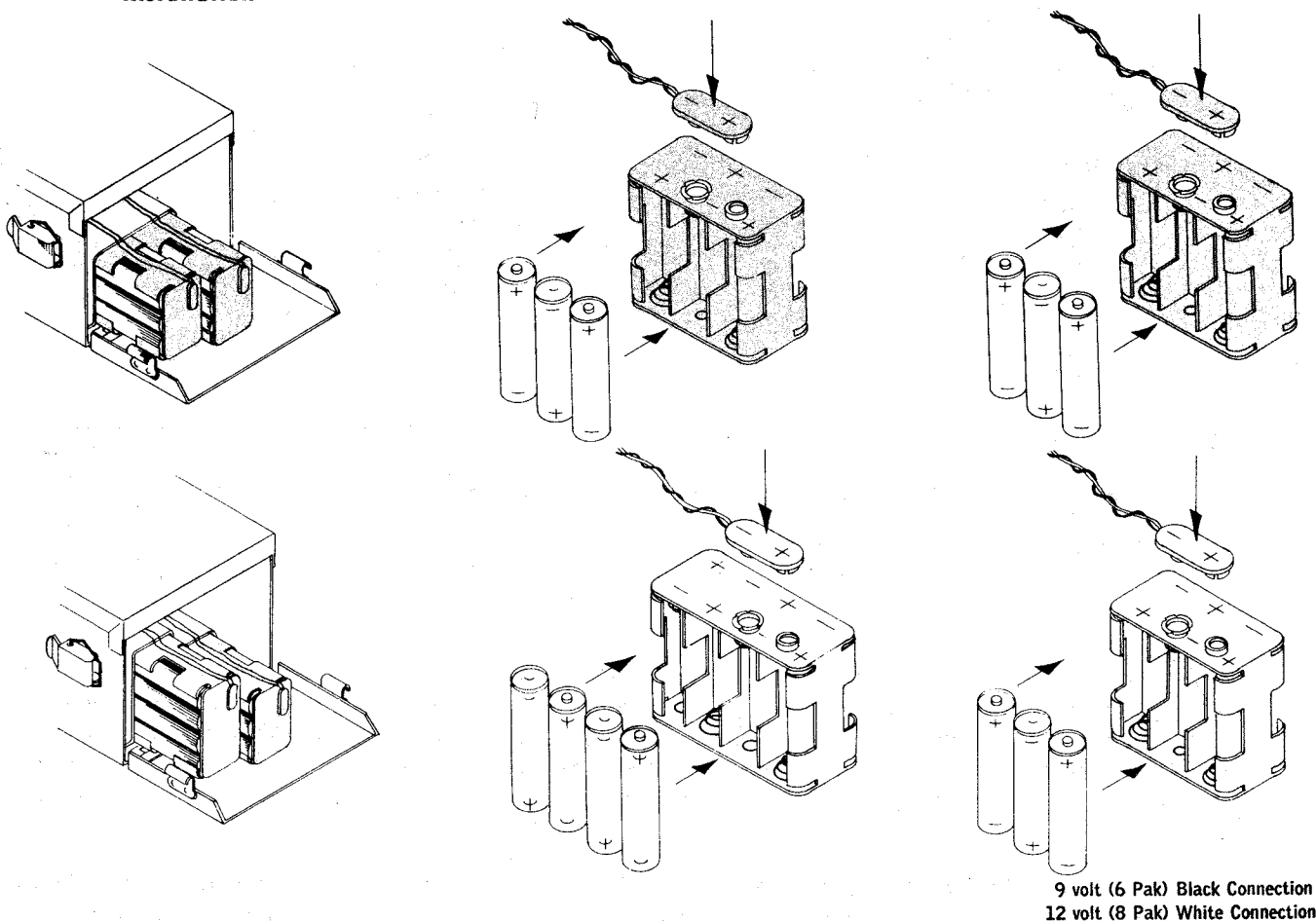
BATTERY-PACK ILLUSTRATION
