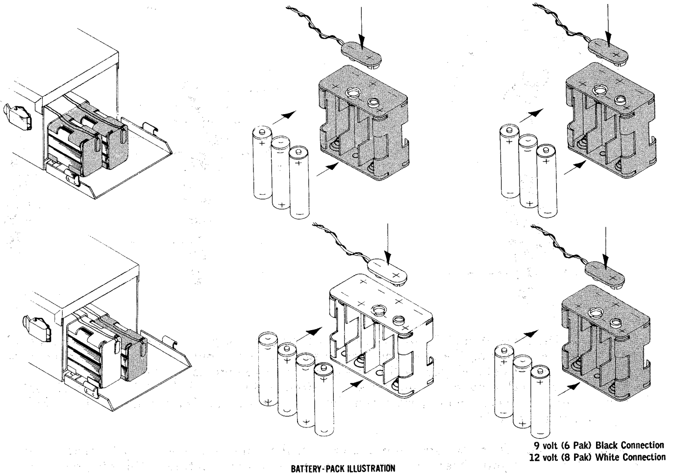
BATTERY-PACK ILLUSTRATION
