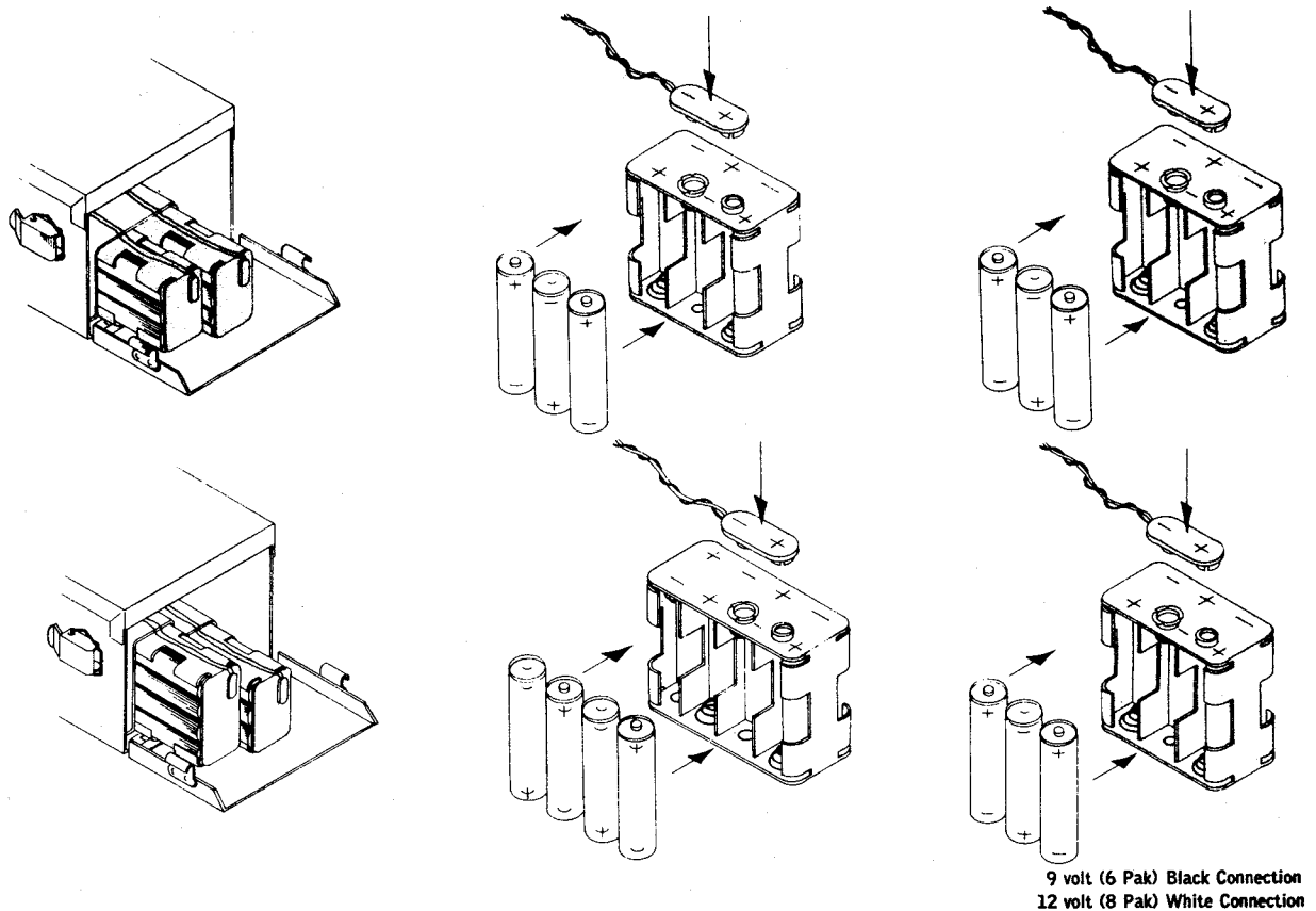
BATTERY-PACK ILLUSTRATION
