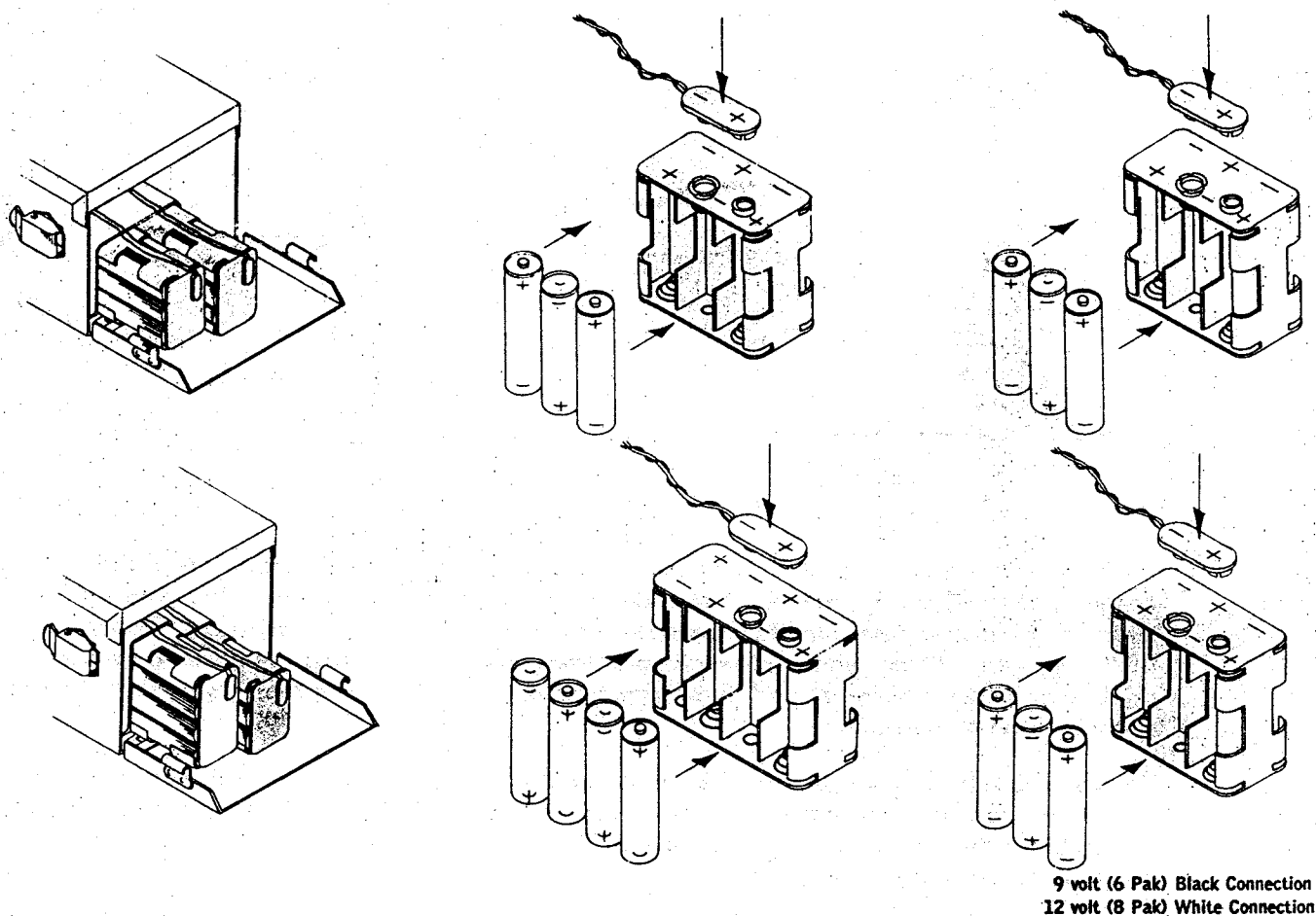
BATTERY-PACK ILLUSTRATION
