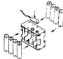
Battery Pack
