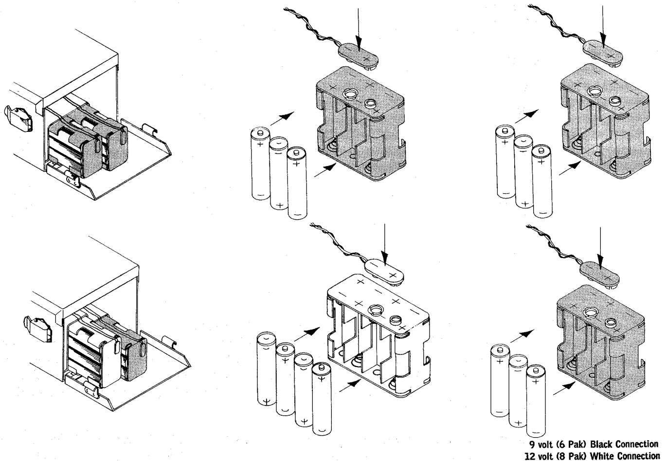
BATTERY-PACK ILLUSTRATION
