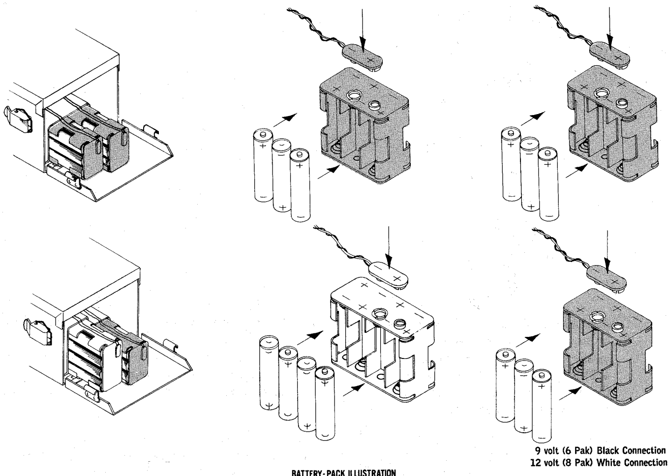
BATTERY-PACK ILLUSTRATION
